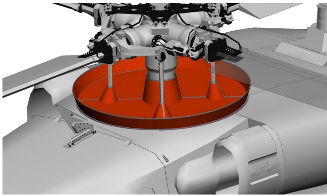
Sikorsky UH-60 Swash Plate FOD Barrier, 3D model
